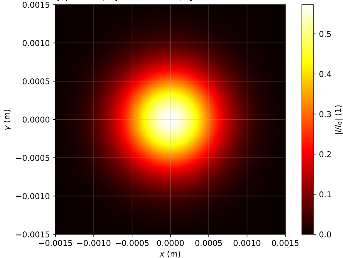
Intensity profile I(x, y, z = 2.070m)/I_0 , P_{in}=0.2P_{cr} , artificial time
